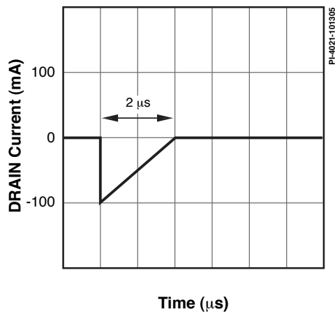
Figure 11. Peak Negative Pulsed DRAIN Current Waveform.
