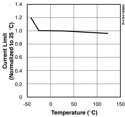
Figure 14. Current Limit vs. Temperature.
