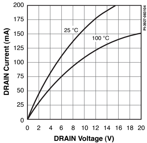
Figure 17. Output Characteristics.
