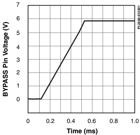
Figure 16. BYPASS Pin Startup Waveform.
