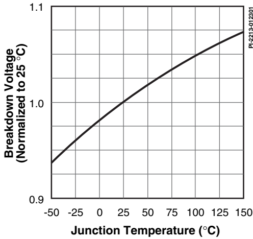
Figure 12. Breakdown vs. Temperature.
